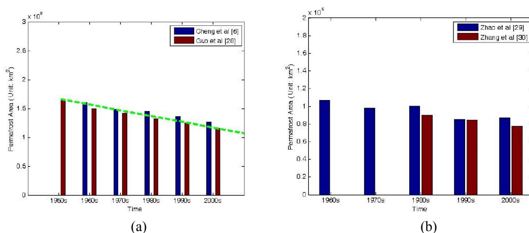
Figure 3. The change in permafrost area of (a) the TP and (b) the Qilian Mountains (north-east TP) from 1960s to 2000s [6, 28-30] with a rate of decrease of 99,000 km 2 per decade [28] for the TP
